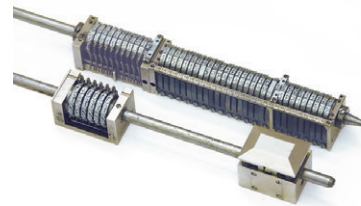
THERM-O-TYPE stocks type high, MICR and Gothic, side plunger activated numbering machines.
