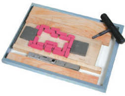
Wood furniture is available in six different widths by 36". Furniture is used to lock up tooling in the letterpress chase.
